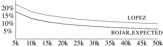
Figure 3: Errors of the different ranking methods discussed in Section 4: Ratio of system pairs where the worst system is ranked better.
