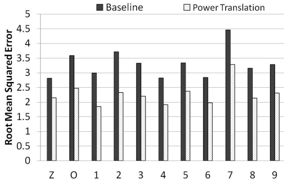
Figure 3: Root mean squared error rate (RMSE) between the reference target duration and the system output for each digit
