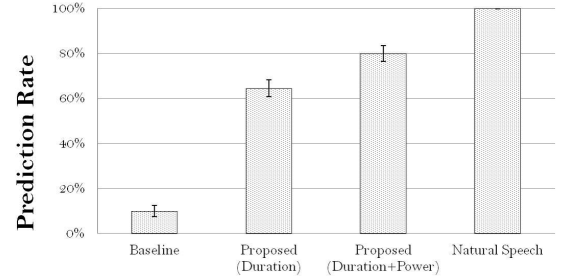
Figure 5: Prediction rate
